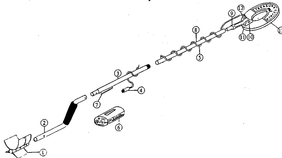
Figure 1. Sterling Assembly Diagram.
